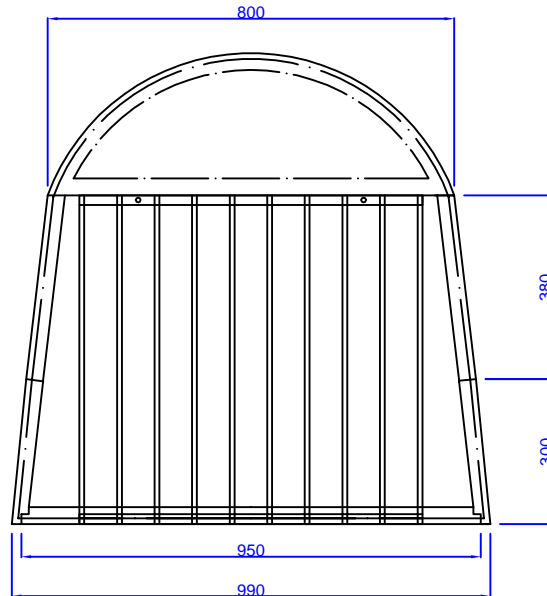
Plan View
