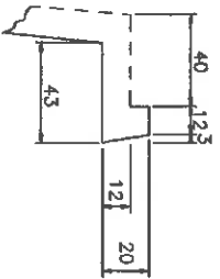
Detail at X
